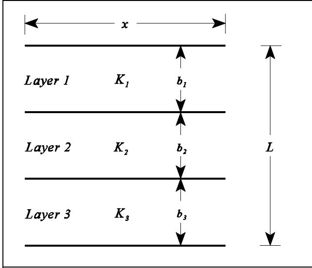
Figure 2-7. Stratified media
